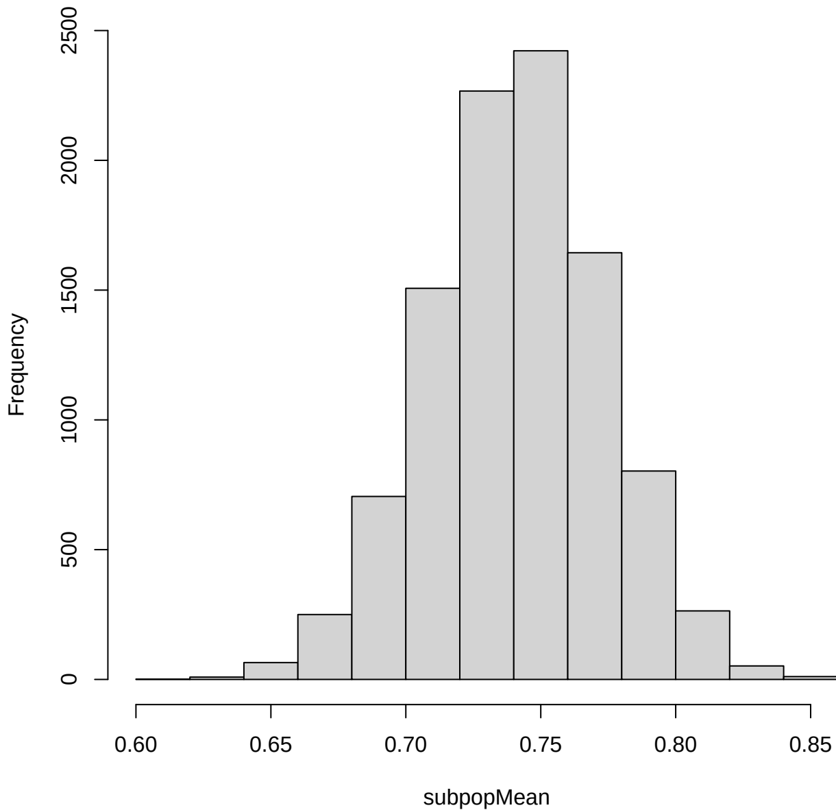
Histogram of subpopMean
