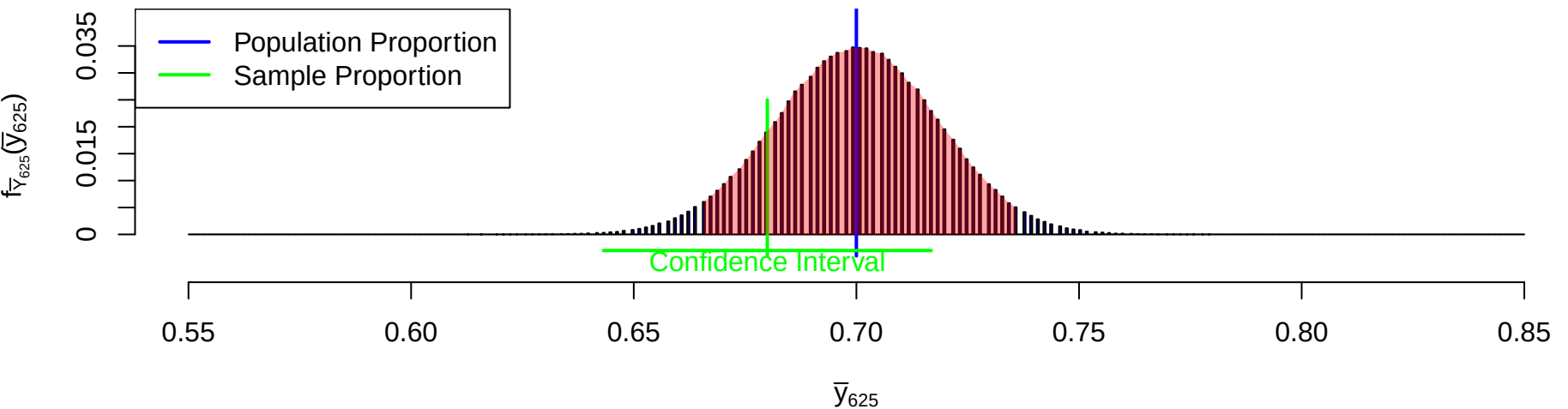
Sampling Distribution of \bar{Y}_{625}
