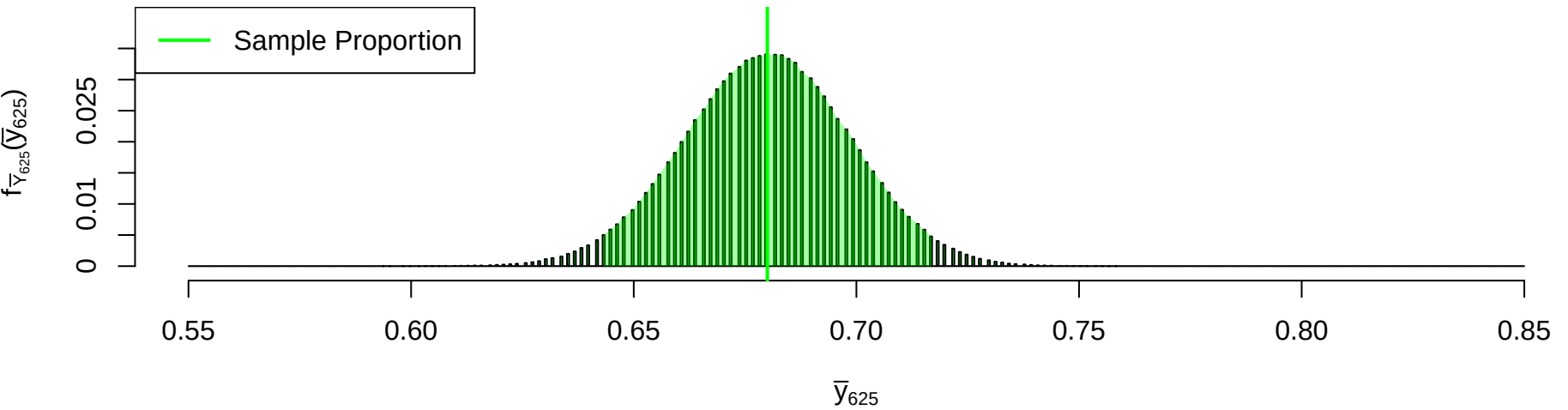
Estimated Sampling Distribution of \bar{Y}_{625}
