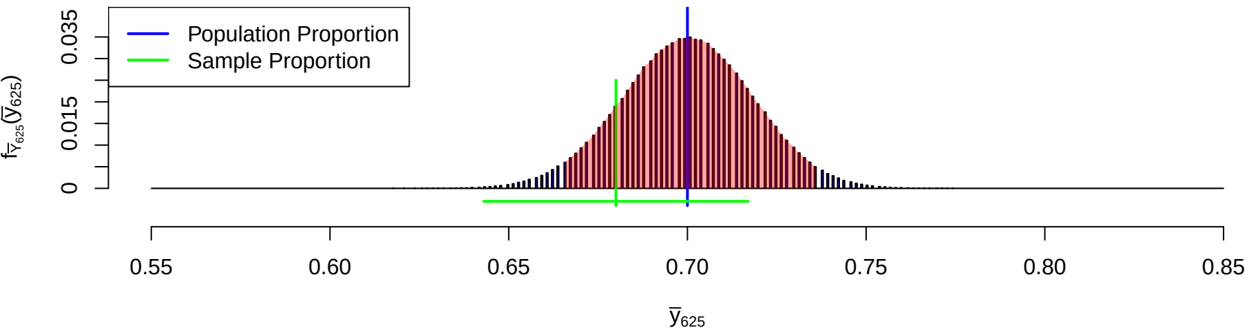
Sampling Distribution of \bar{Y}_{625}
