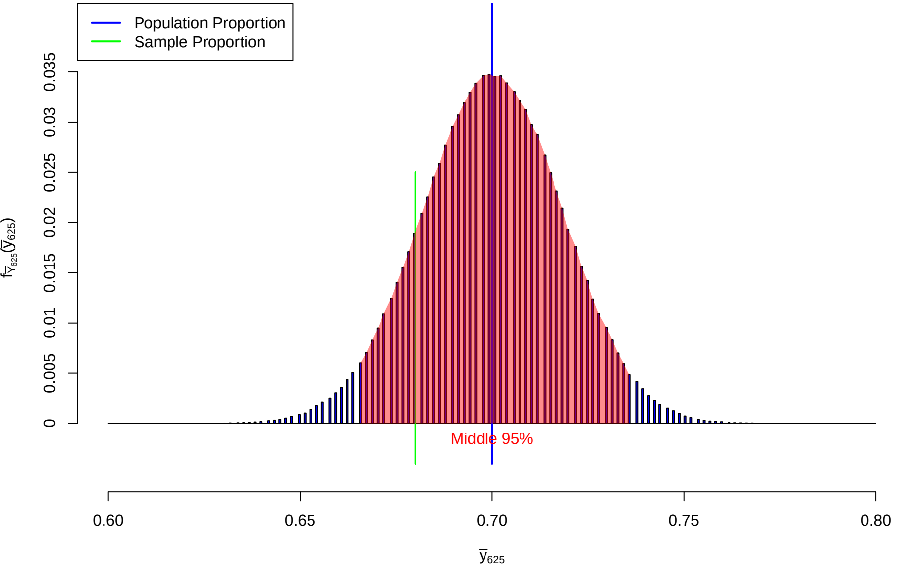
Sampling Distribution of \bar{Y}_{625}
