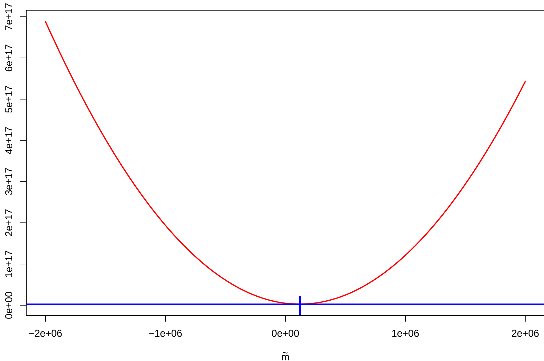
Sum of Squared Residuals
