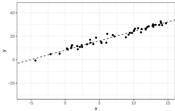
Figure 4: Scatterplot of x and y
