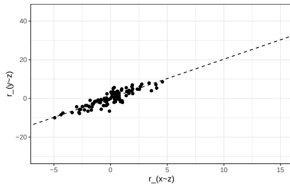
Figure 5: Scatterplot of residuals from lm(x \sim z) and lm(y \sim z)
