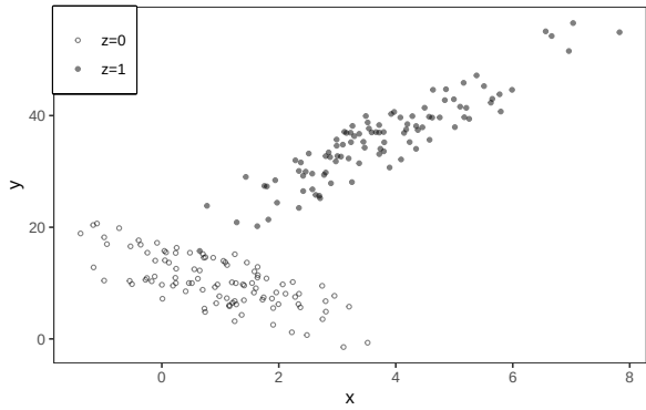
Figure 6: Scatterplot 1
