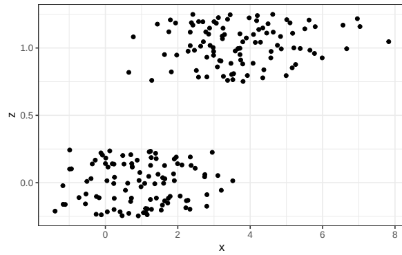
Figure 7: Scatterplot 2 (jittered)
