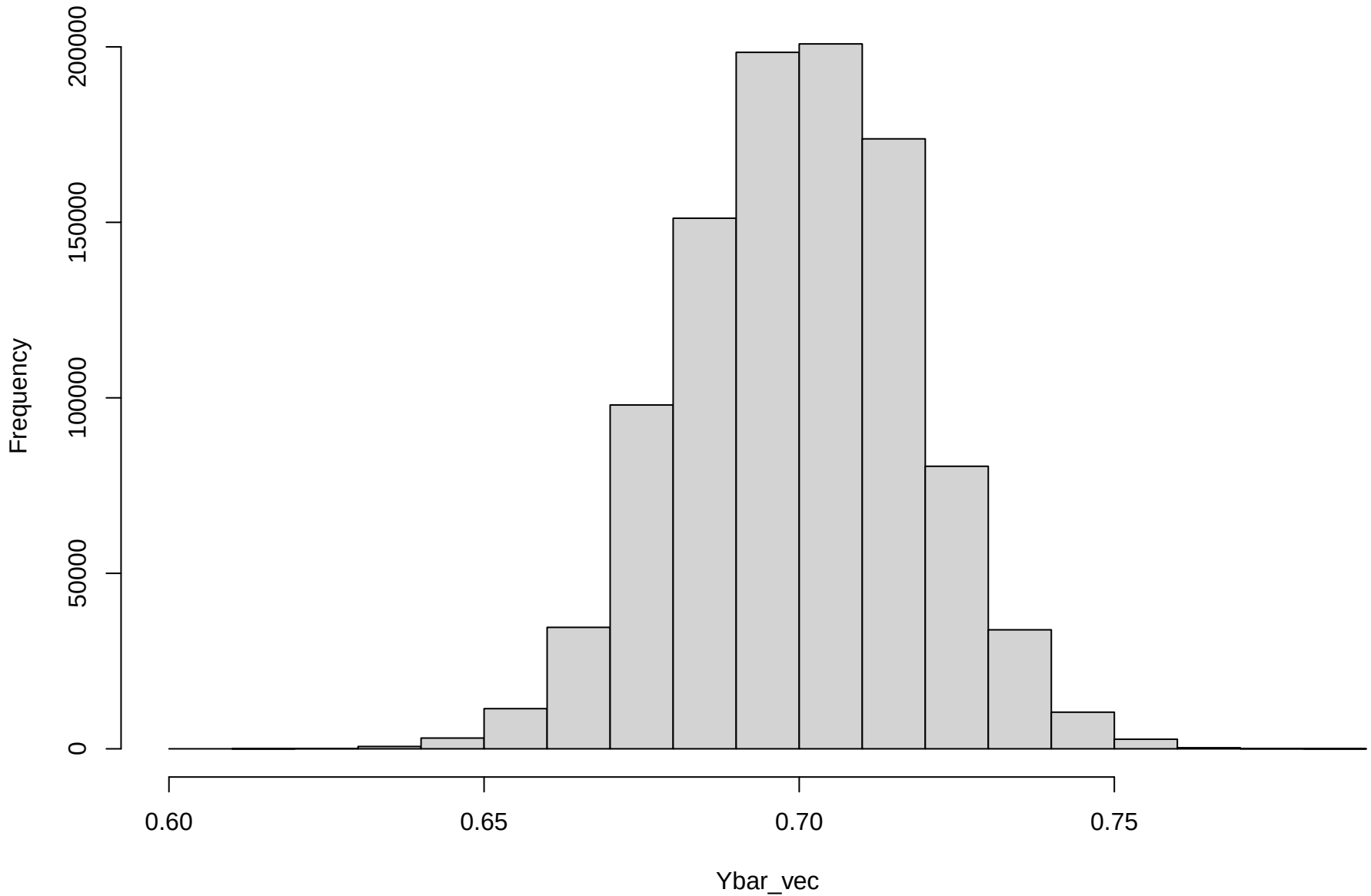
Histogram of Ybar_vec
