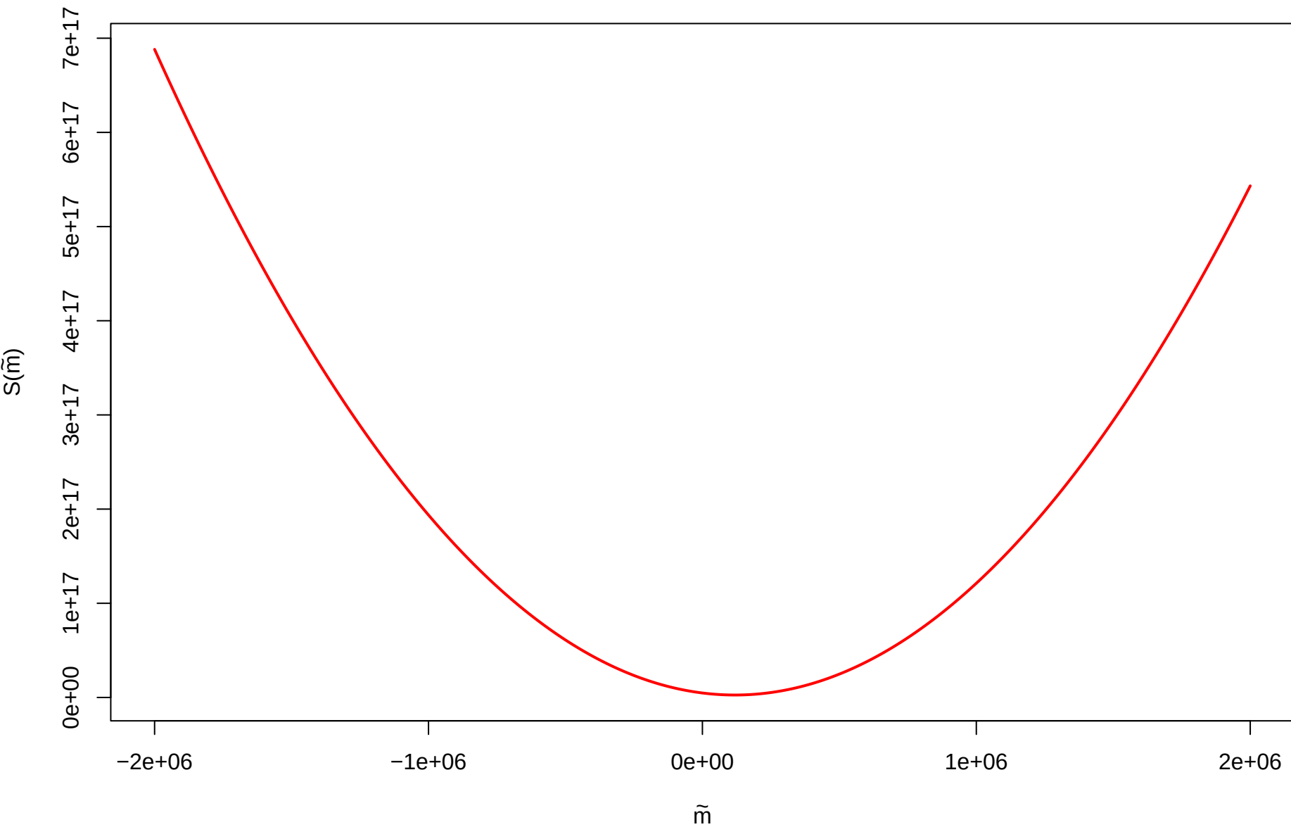
Sum of Squared Residuals
