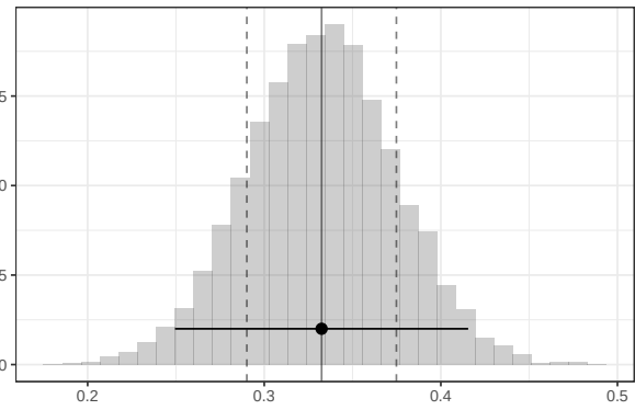
Figure 4: Histogram of the \beta_1 's elements
