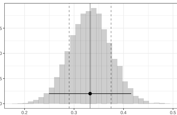
Figure 3: Histogram of the beta_0's elements
