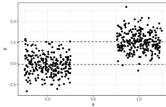
Figure 2: Jittered Scatterplot of X and Y
