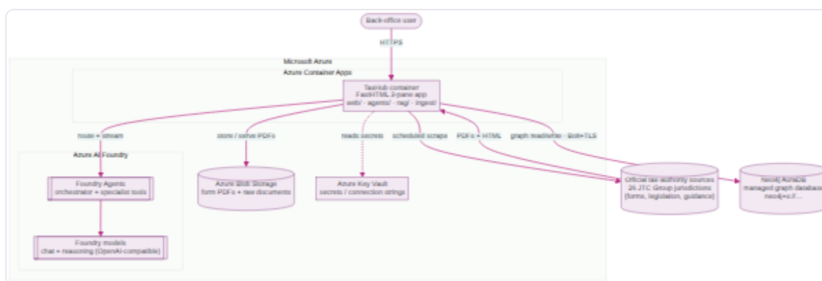
TaxHub on Azure — target production architecture
