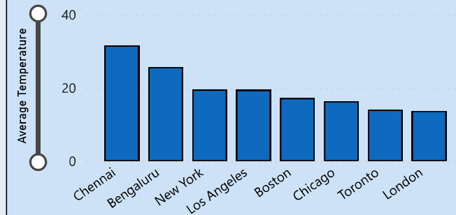
Average Temperature by City
