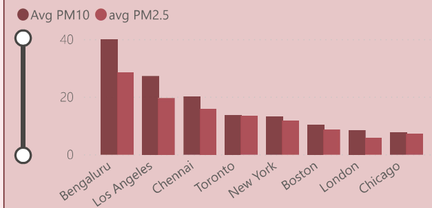
Average PM10 Vs Average PM2.5 by city
