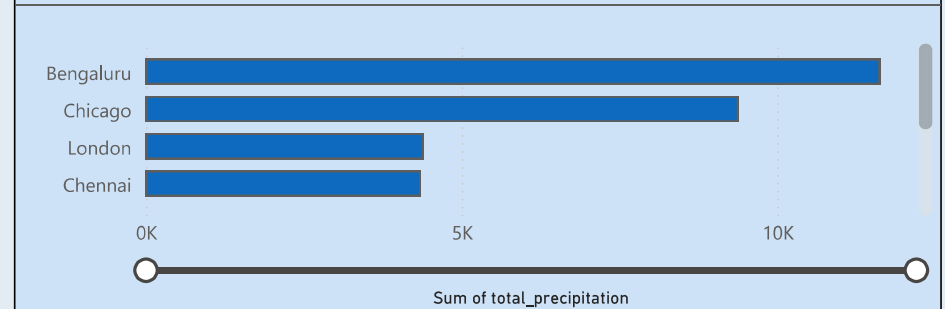
Total_precipitation by city
