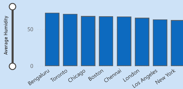
Average Humidity by City
