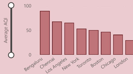
Average AQI by city
