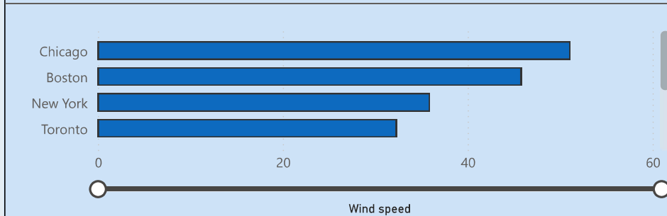
Max wind_speed by city
