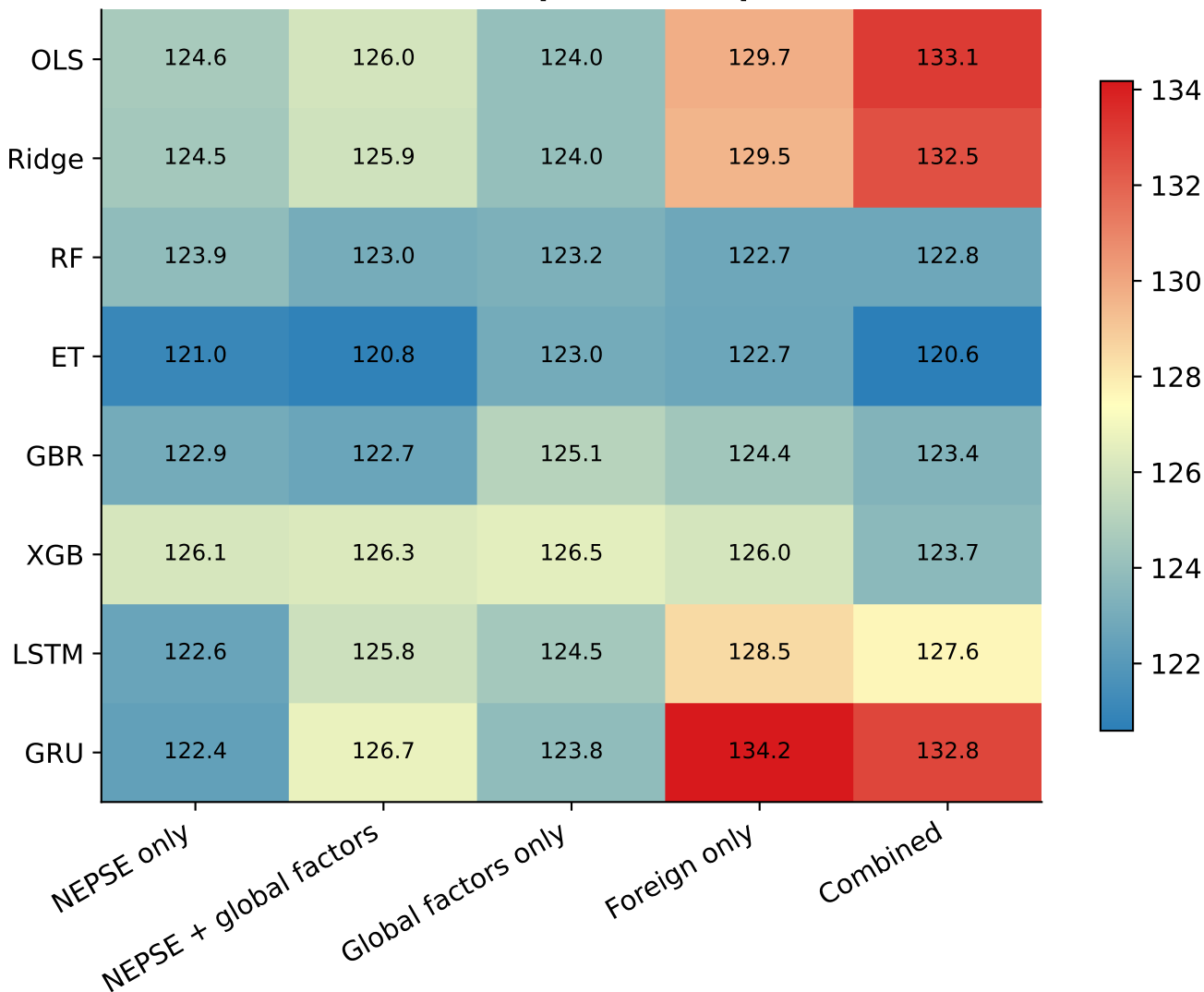
Out-of-sample RMSE (bps)
