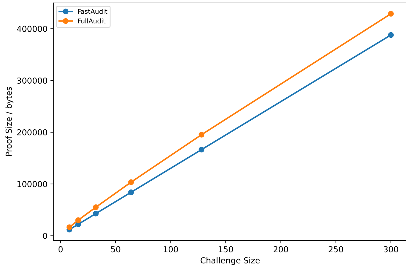
Serialized Proof Size
