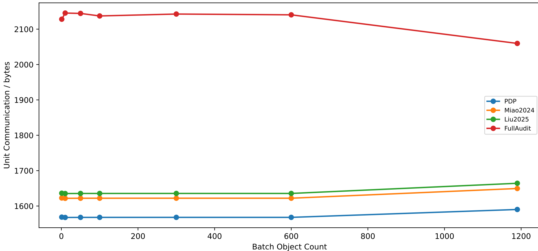
Full-Scale Batch Communication
