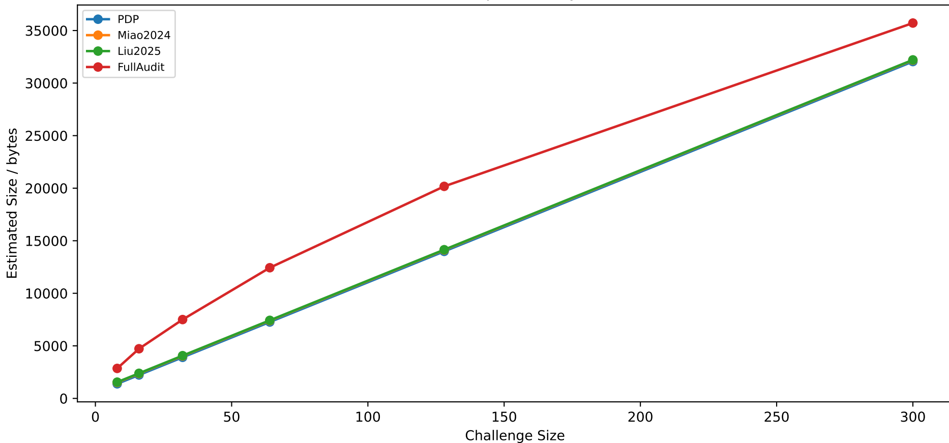
Full-Scale Compact Binary Proof Size
