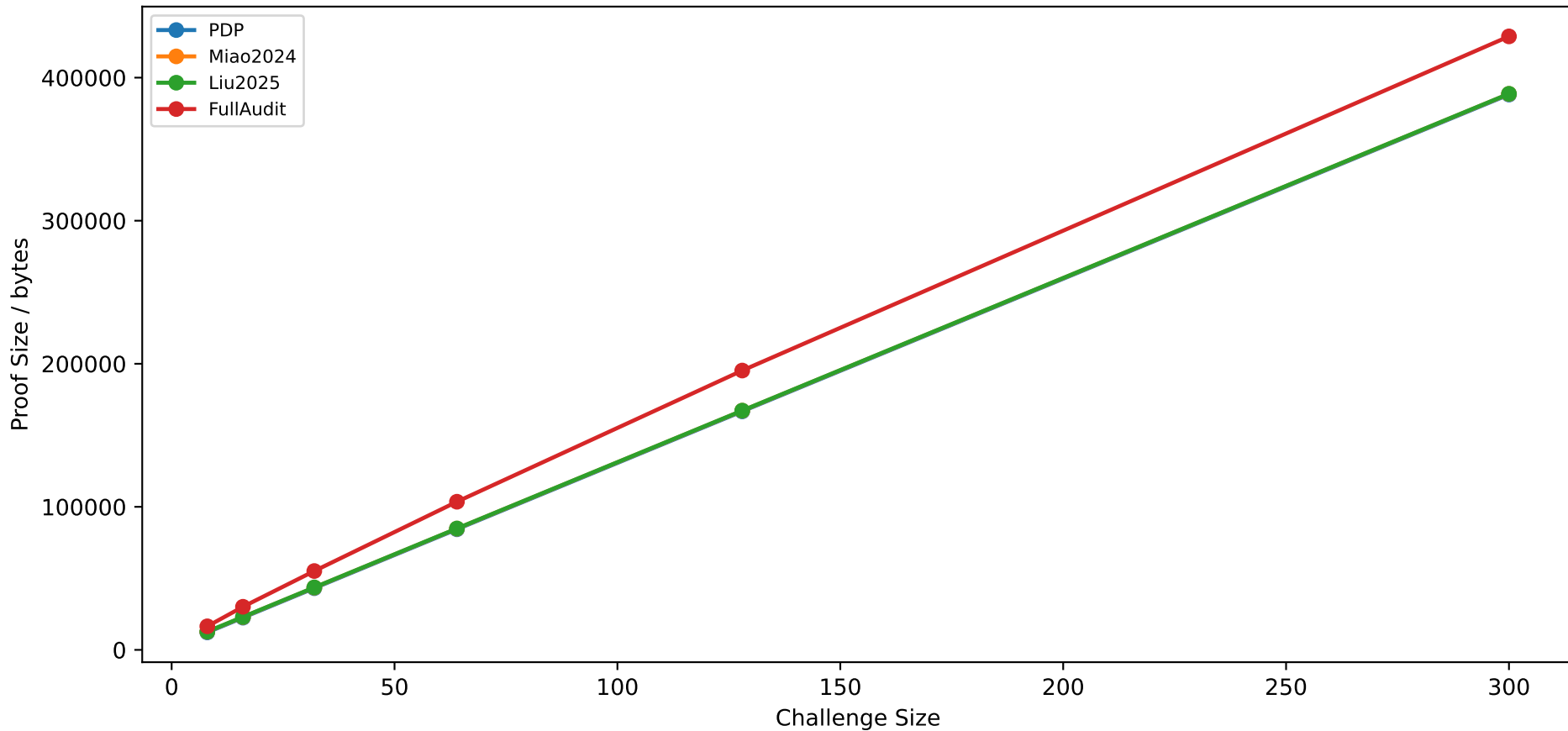
Full-Scale Serialized Proof Size
