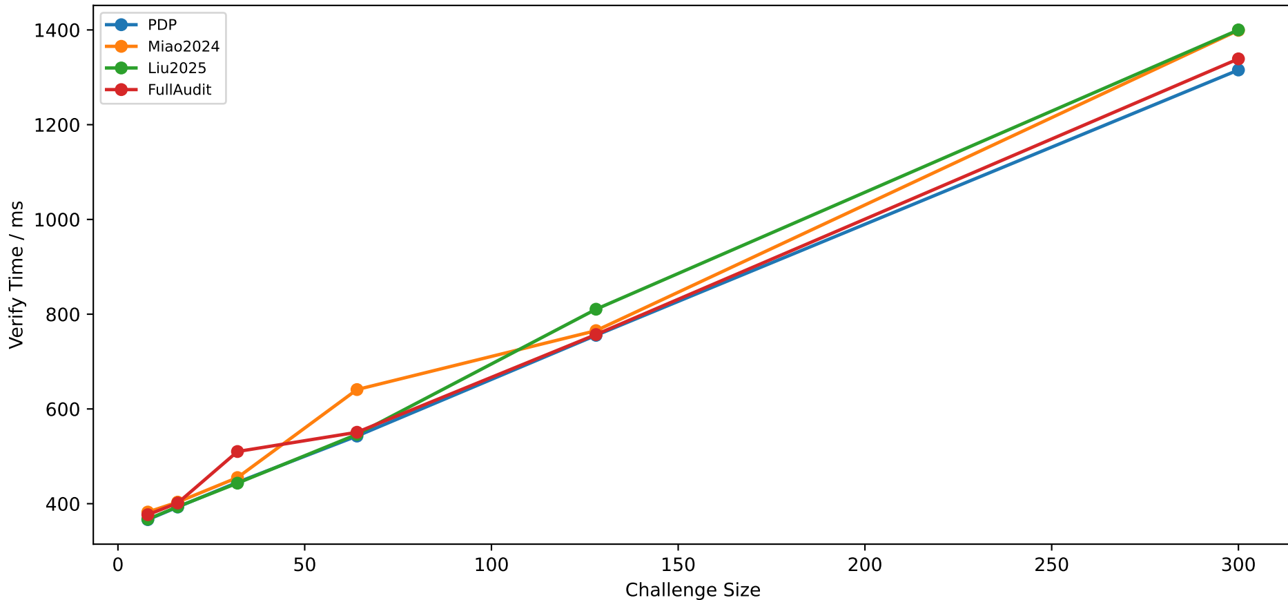
Full-Scale Online Verification Time
