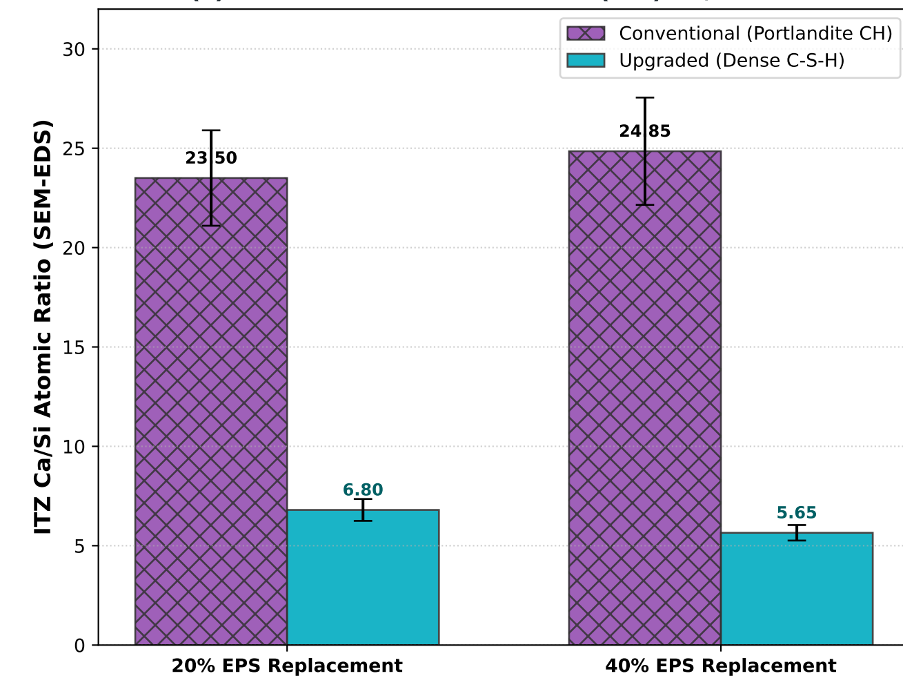
(c) Interfacial Transition Zone (ITZ) Ca/Si Ratio
