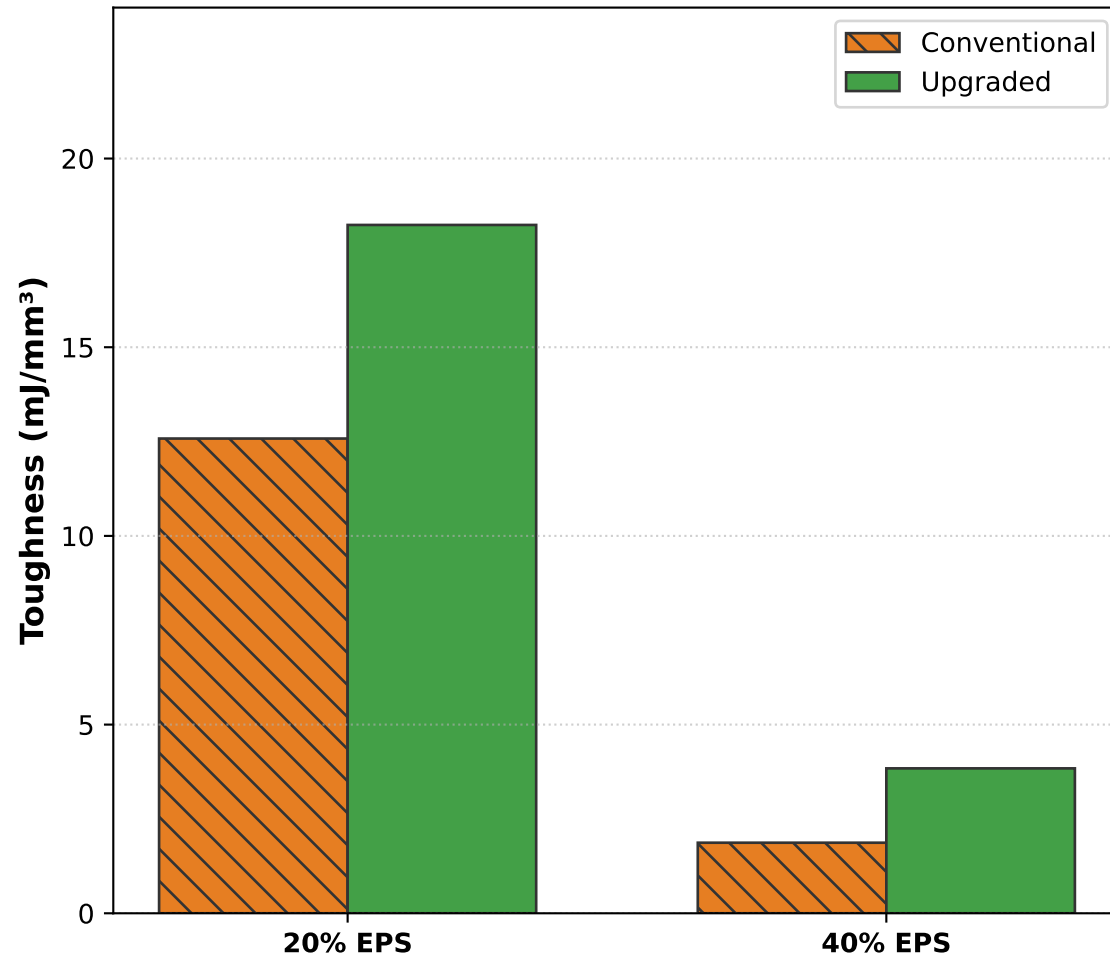
2. Post-Crack Fracture Energy
