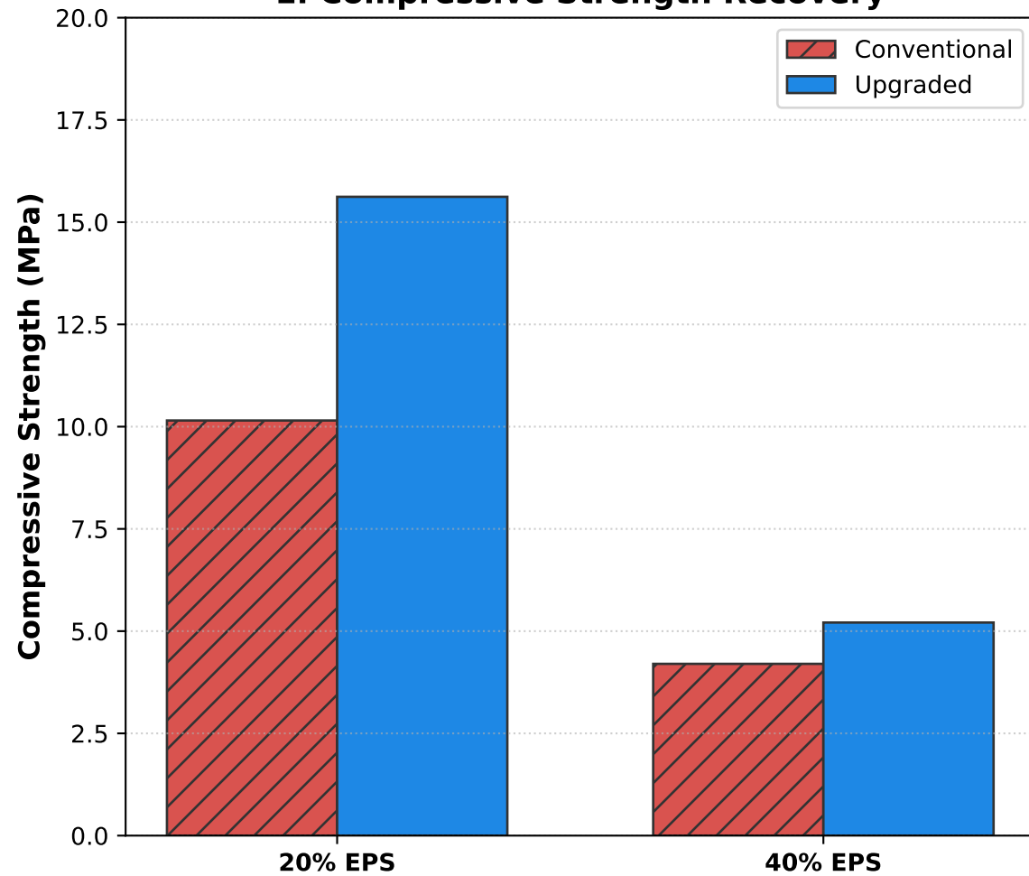
1. Compressive Strength Recovery
