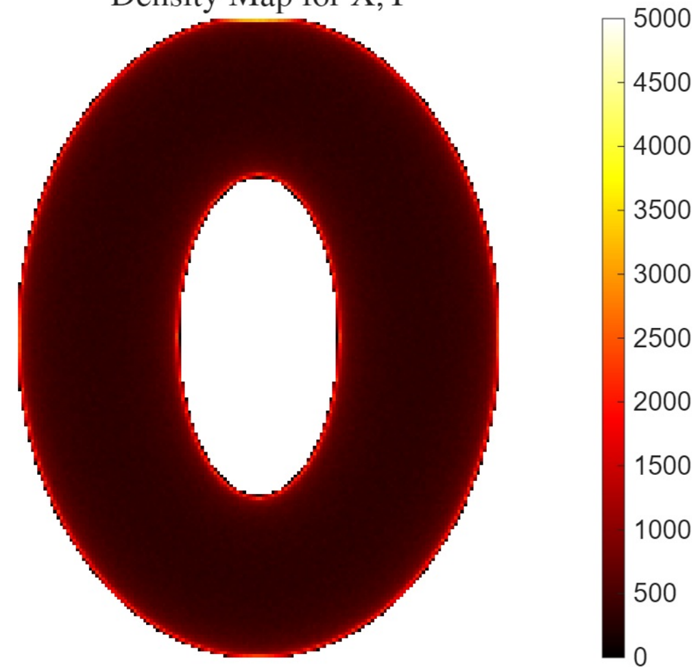
Torus Density Map for X,Y
