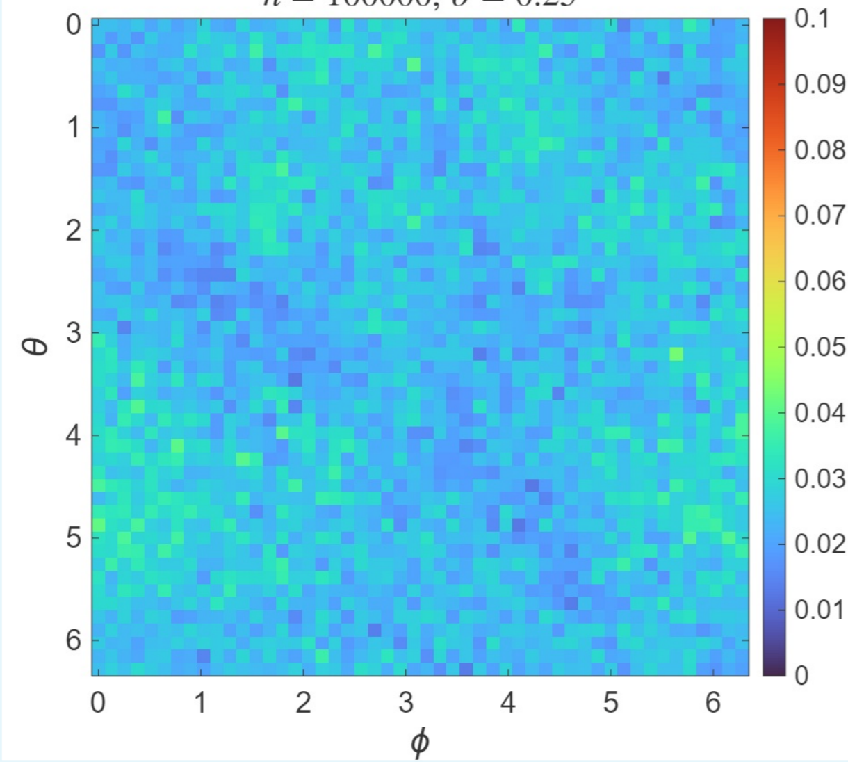
\phi vs \theta Density Heatmap n = 100000, \sigma = 0.25
