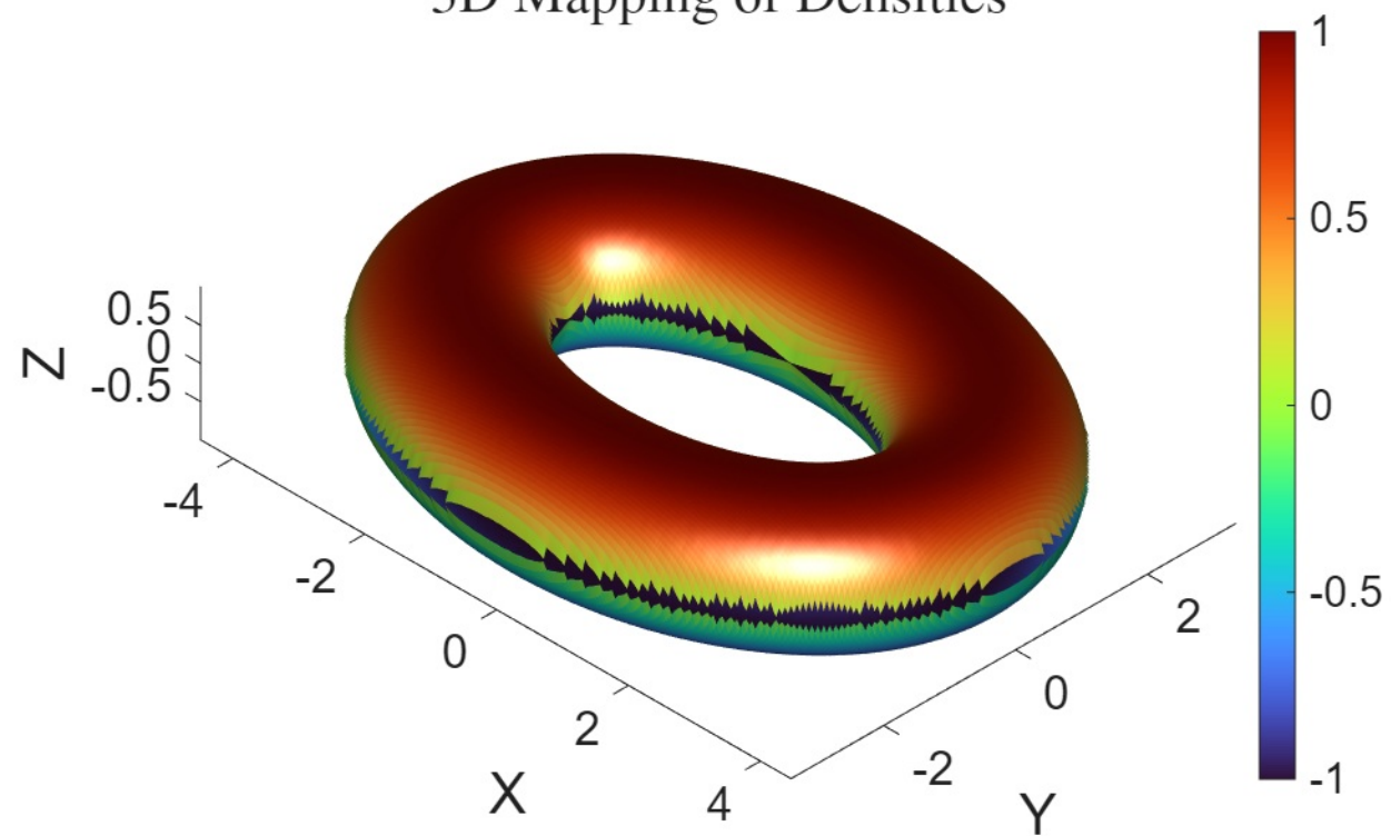
Torus 3D Mapping of Densities
