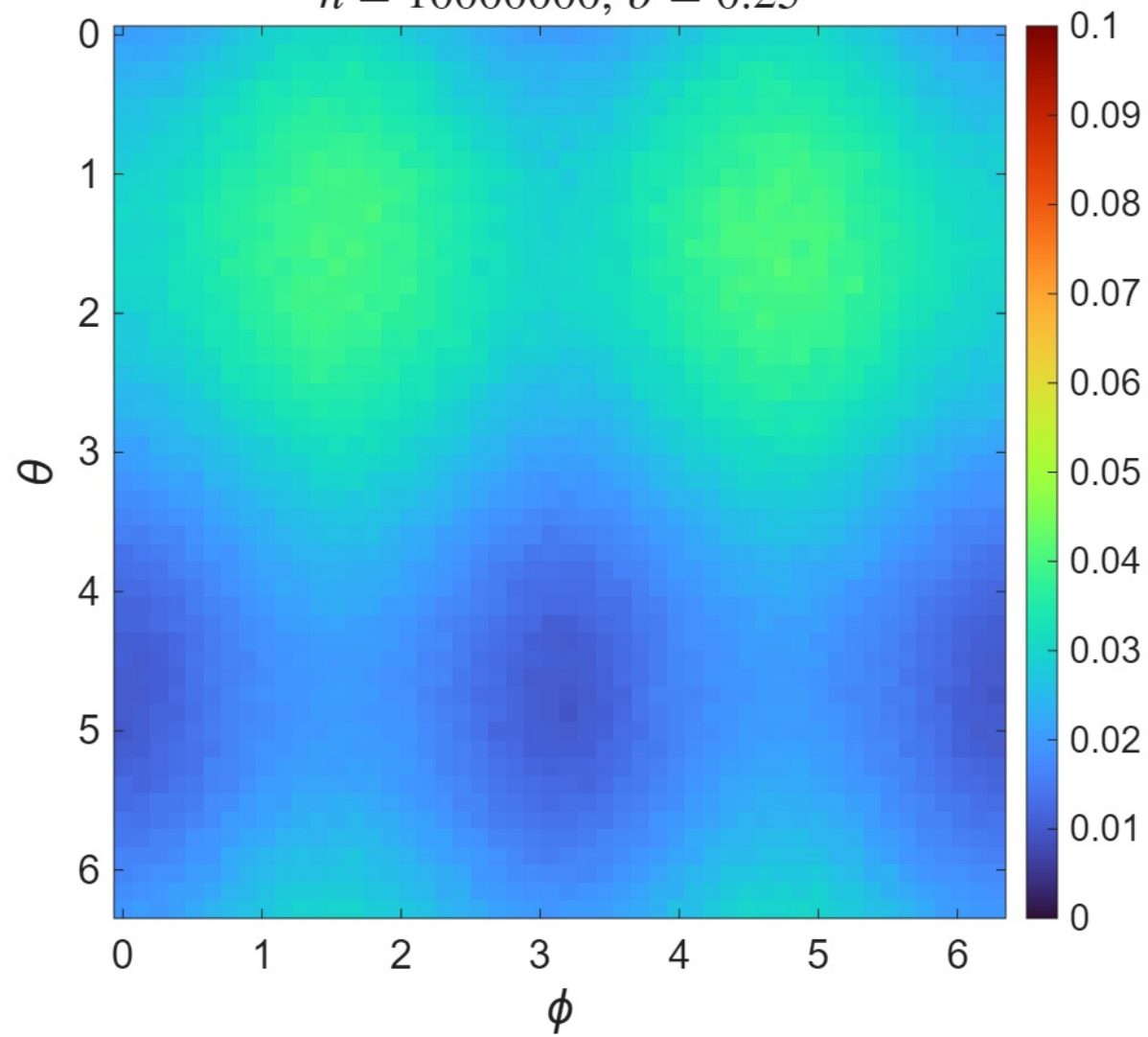
\phi vs \theta Density Heatmap n = 10000000, \sigma = 0.25
