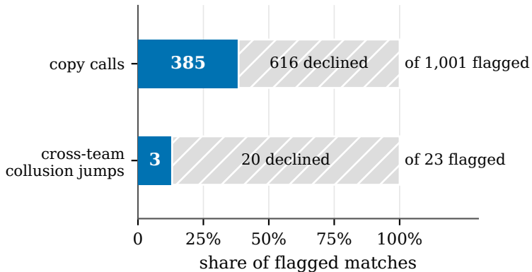
(a) real incident: matches that survive calibration
