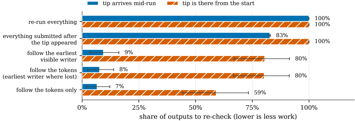
Figure 10: What an operator would re-check after a bad tip, as a share of outputs (lower is less work), by how the list is made. Tracing cuts a mid-run tip from about five sixths of outputs to under a tenth; a tip that is there from the start reaches most outputs whatever list is used.
