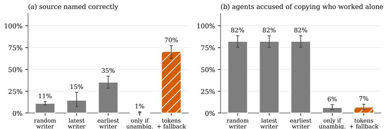
Figure 8: Benchmark baselines on the tagged runs: (a) copying agents whose source is named correctly; (b) agents that worked alone but were accused of copying. The first three rules blame an earlier writer whenever one exists, so (b) is high for them by construction.
