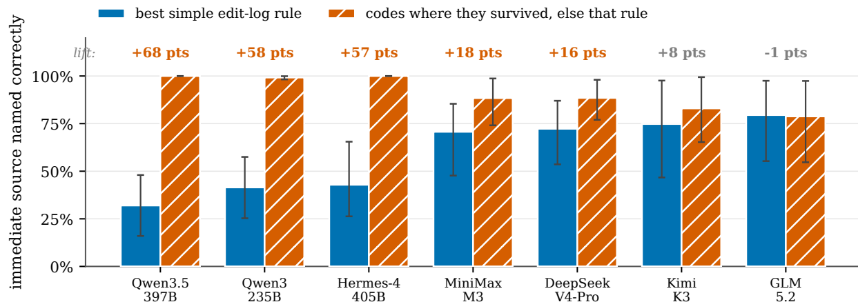
Figure 7: How often the immediate source is named correctly, by model: the best simple edit-log rule for each run against the token (with that rule as fallback where the token was lost). The number above each pair is the lift in points; it is large where the token survives (Figure 6).
