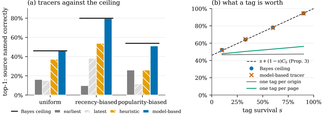
Figure 5: The theory against a simulator with a known answer. (a) Top-1 accuracy of tracers against the exact Bayes ceiling (black bars) under three copy rules. (b) What a tag is worth: the ceiling and the model-based tracer follow s + (1 - s)C_0 for version-unique tags; tags per origin or per page barely help.
