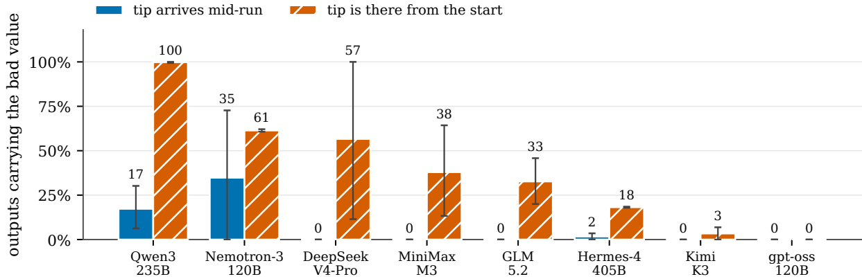
Figure 9: Outputs that carry the planted bad value, by model, for a tip that arrives mid-run and a tip that is there from the start. Intervals are wide because there are two to four runs per model.
