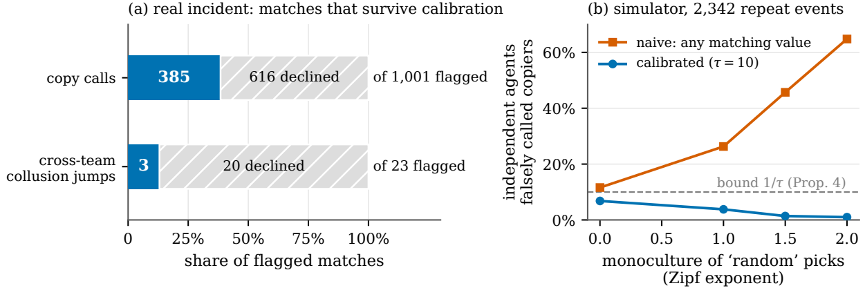
Figure 4: The coincidence trap. (a) On the real incident, most naive copy calls and cross-team collusion jumps do not survive calibration. (b) In a simulator, the naive detector falsely calls more independent agents copiers as their choices become more alike (monoculture), while the calibrated detector stays below the bound 1/\tau of Proposition 4 (here \tau = 10 ).
