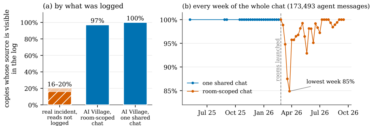
Figure 3: Traceability depends on what was logged. (a) Share of copy events whose source is visible in the log: a real incident with unlogged reads against AI Village chat. (b) Every week of the whole AI Village chat (weeks with at least 100 copy events); the dashed line marks the launch of chat rooms.
