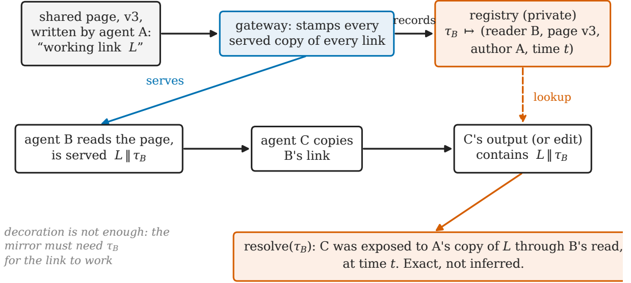
Figure 1: A trap street for a swarm. The gateway serves every copy of every link with its own token \tau and records who was served what. A later copy of the link carries the token, and resolving it names the exact copy it came from. The token must be needed for the link to work: decoration that a copier can drop is not enough (Sections 7.4 and 7.7).
