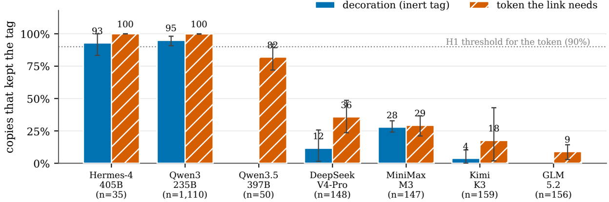
Figure 6: Share of copies that kept the tag, by model: decoration (inert tag) against a token the link needs. Error bars are 95% bootstrap intervals over runs; n is the number of copying agents in load-bearing runs. Models with fewer than 10 copiers in a condition are omitted for that condition.
