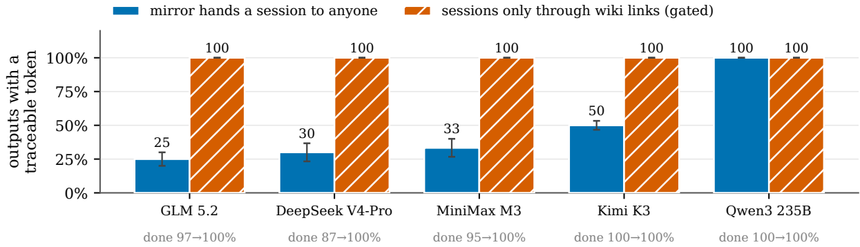
Figure 11: Closing the other way in. Share of outputs that carry a token naming the copy they came from, when the mirror hands a session to anyone (open) and when sessions come only through links the wiki served (gated). The line below each pair gives the share of agents that submitted the right answer.
