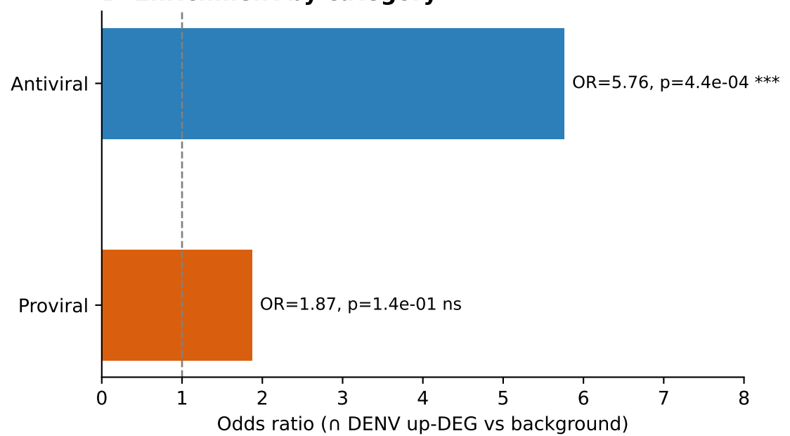
B Enrichment by category
