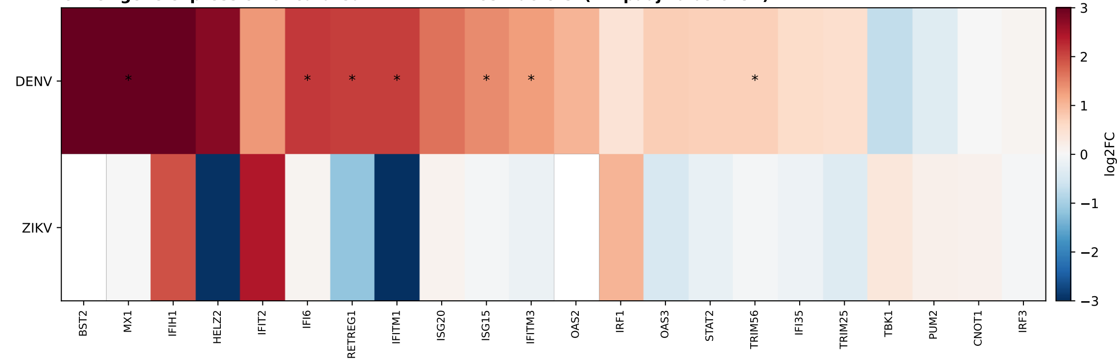
C Per-gene expression of curated ANTIVIRAL host factors (* = padj<0.05 & UP)
