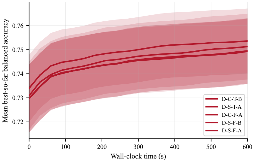
Convergence at 600s budget
