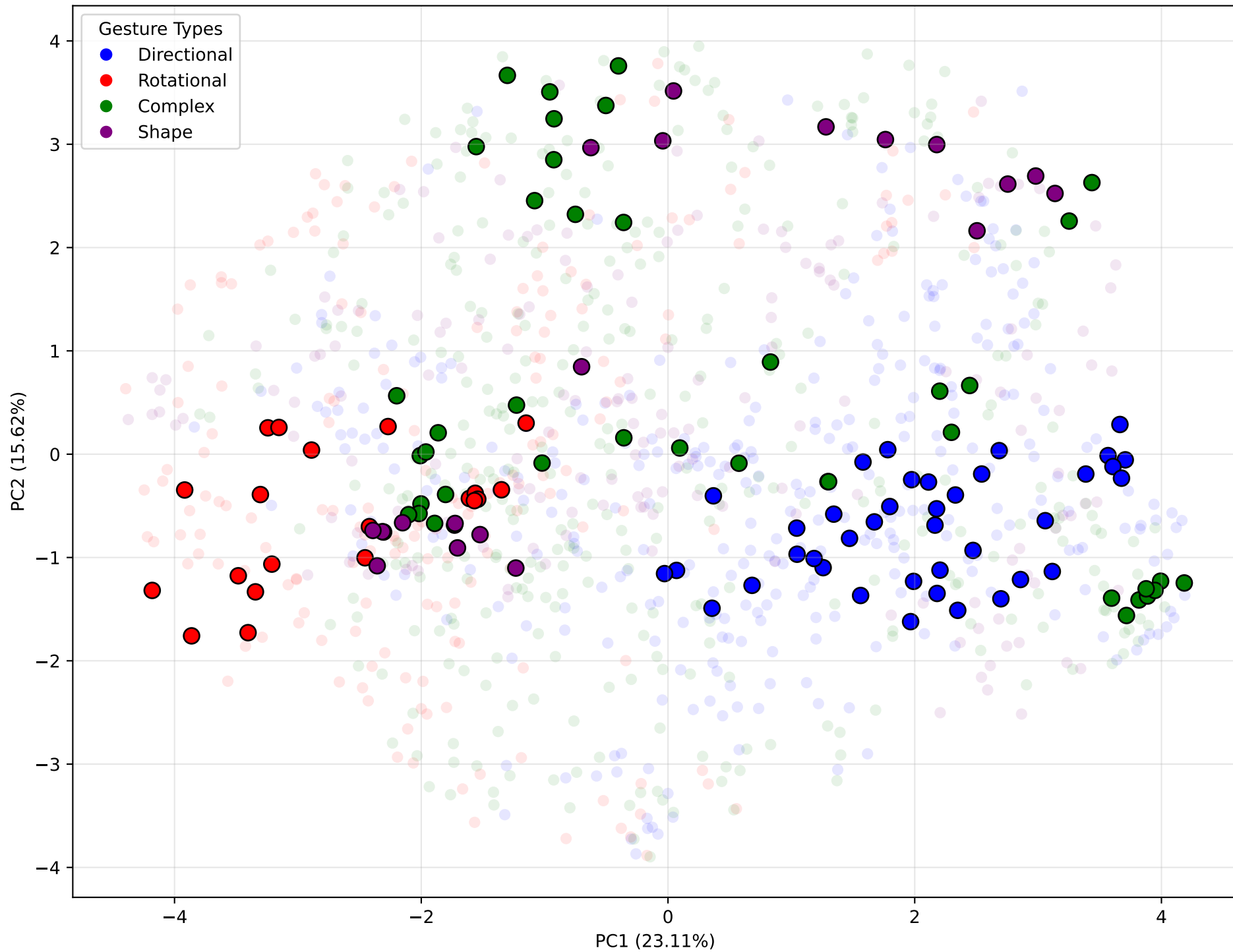
PCA of Selected Representative Samples
