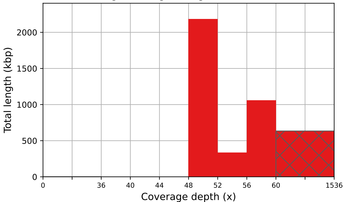
contigs coverage histogram (bin size: 4x)
