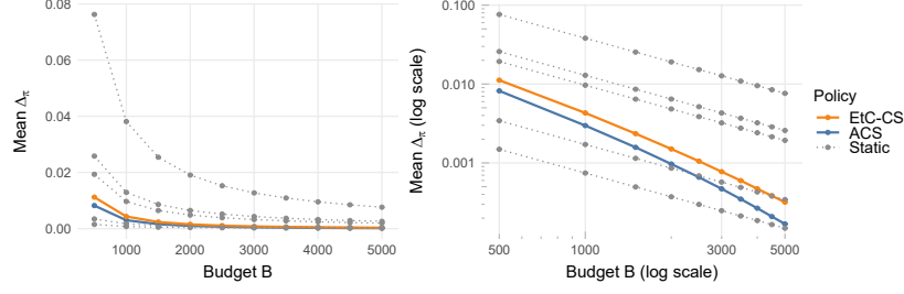
Figure 5: Mean excess variance across budget
