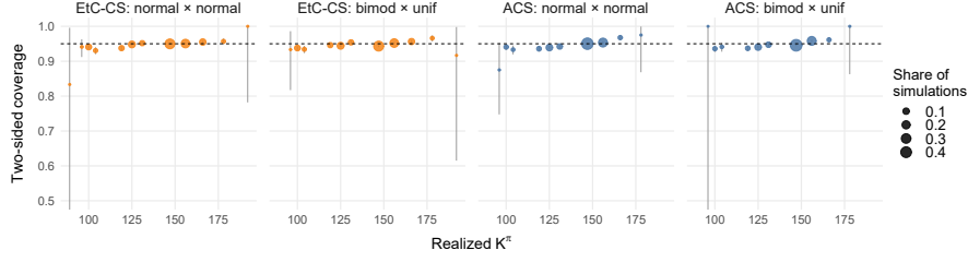
Figure 7: Design-conditional coverage of \hat{\mu}_{K_B^\pi, N_B^\pi} \pm 1.96 \hat{b}_{K_B^\pi, N_B^\pi} / \sqrt{K_B^\pi}
