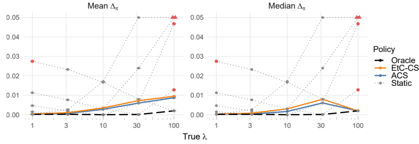
Figure 4: Excess variance across \lambda_0
