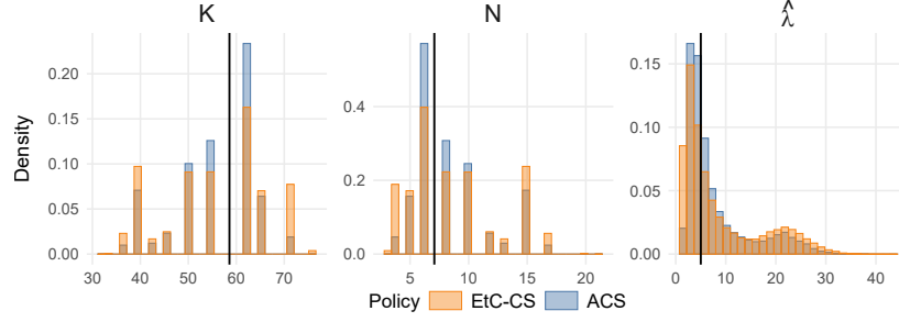
Figure 3: Design (K_B^\pi, N_B^\pi) and pilot estimate \hat{\lambda}_{pB} for EtC-CS and ACS
