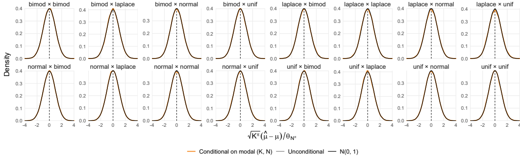
Figure 14: Empirical density of the design-conditional statistic \sqrt{K_B^\pi}(\hat{\mu}_{K_B^\pi, N_B^\pi} - \mu)/\theta_{N_B^\pi} at the modal design across symmetric error distributions
