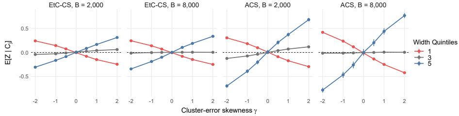
Figure 10: Design-conditional expectation \mathbb{E}[Z_B^\pi | C_j] as a function of \text{Skew}(u_k)
