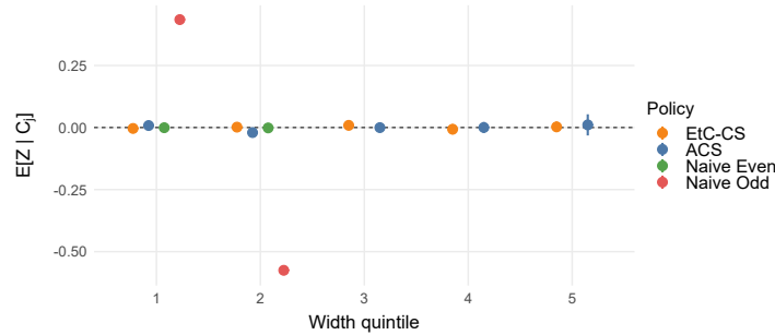
Figure 8: Design-conditional expectation \mathbb{E}[Z_B^\pi \mid C_j] over width quintiles
