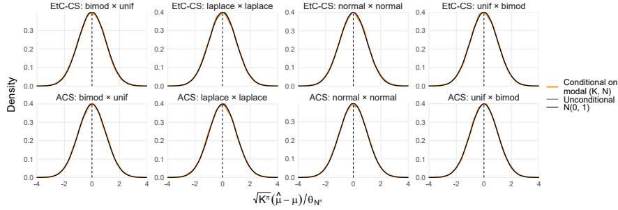
Figure 6: Empirical density of Z_B^\pi / \theta_{N_B}^\pi at the modal design and unconditionally under symmetry
