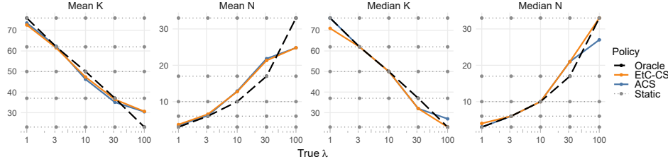
Figure 13: Mean and median terminal design (K_B^\pi, N_B^\pi) across \lambda_0
