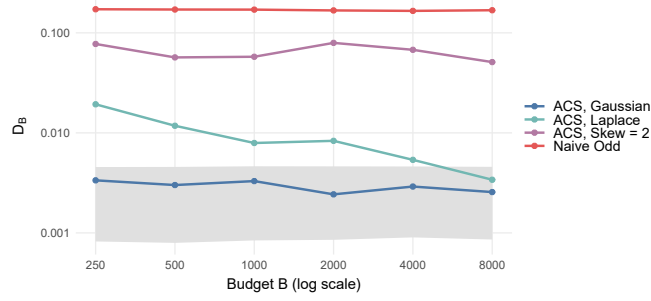
Figure 9: Maximal discrepancy between the conditional and normal characteristic functions
