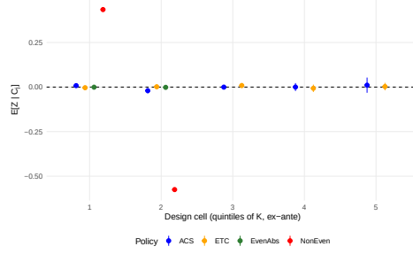
Figure 8: Design-conditional expectation \mathbb{E}[Z_B^\pi | C_j] over width quintiles
