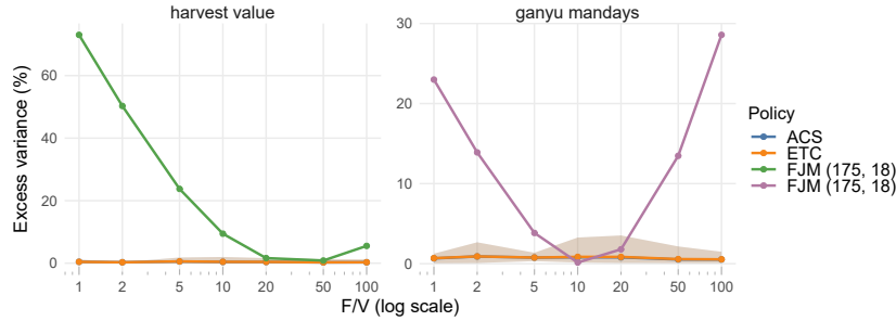
Figure 12: Excess variance across cost ratios
