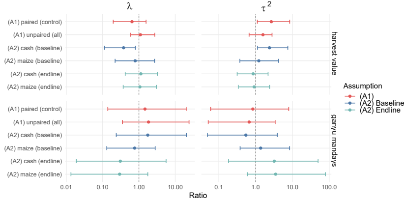
Figure 15: Variance-homogeneity tests
