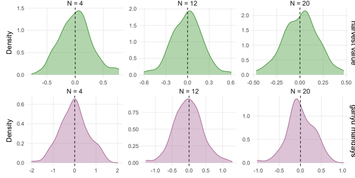
Figure 16: Density of the centered residuals \hat{M}_{k,N}
