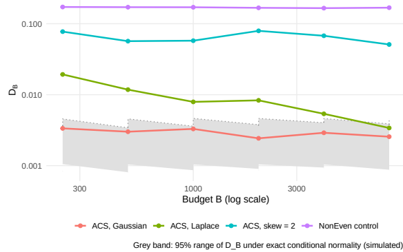
Figure 9: Maximal discrepancy between the conditional and normal characteristic functions
