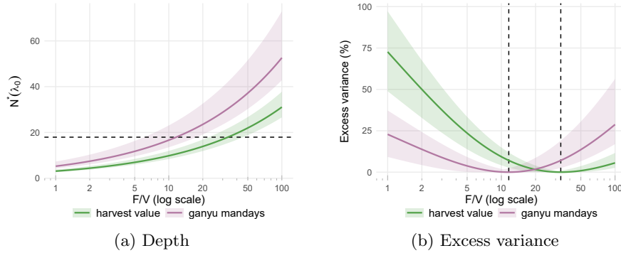
Figure 11: Realized FJM design against the oracle across F/V cost ratios
