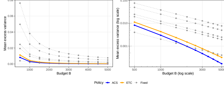
Figure 5: Mean excess variance across budget
