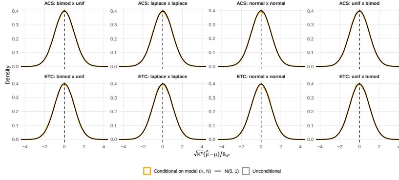
Figure 6: Empirical density of Z_B^\pi / \theta_{N_B^\pi} at the modal design and unconditionally under symmetry Notes: Distribution of u_k (left) and \varepsilon_{ki} (right). Distributions considered: Bimodal-Uniform, Laplace-Laplace, Normal-Normal, Uniform-Bimodal. 10^5 replications. \mu = 0 , \omega = (1, 5) , B = 2,000 , F = 20 , V = 2 .
