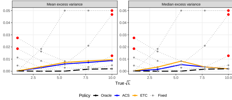
Figure 4: Excess variance across \lambda_0
