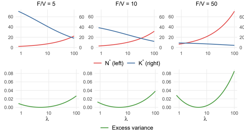
Figure 1: Design and excess variance under \lambda misspecification
