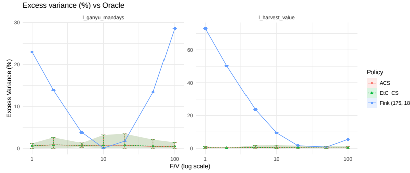
Figure 12: Excess variance across cost ratios
