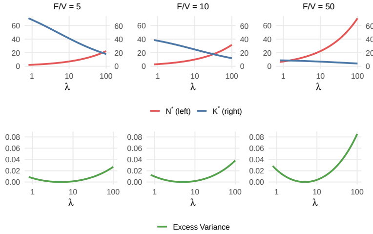
Figure 1: Design and Excess Variance under \lambda Misspecification
