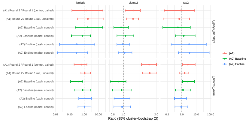
Figure 15: Variance-homogeneity tests
