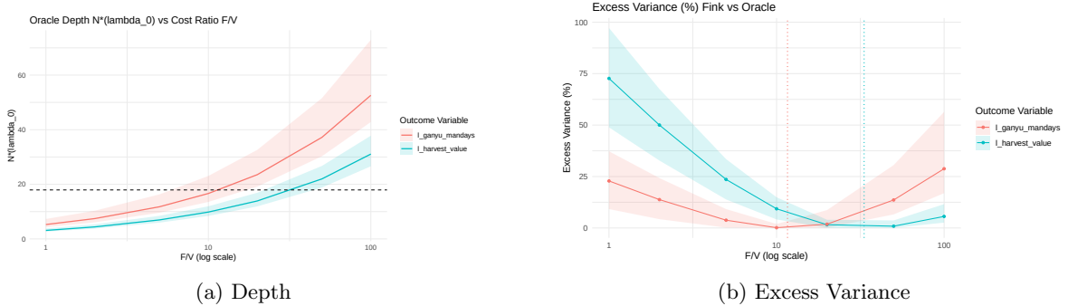
Figure 11: Realized FJM design against the oracle across F/V cost ratios
