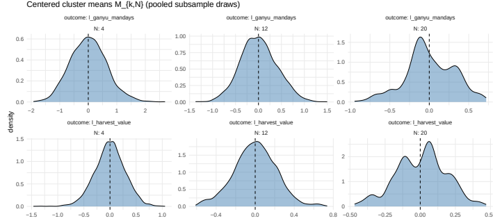
Figure 16: Density of the centered residuals \hat{M}_{k,N}
