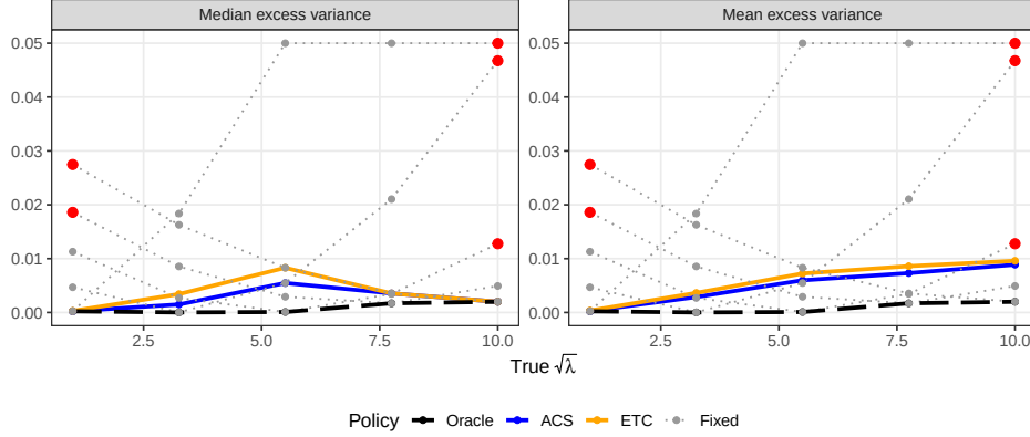
Figure 4: Excess Variance across \lambda_0
