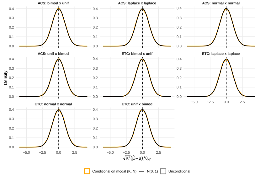
Figure 6: Empirical density of the design-conditional statistic \sqrt{K_B^\pi}(\hat{\mu}_{K_B^\pi, N_B^\pi} - \mu) / \theta_{N_B^\pi} at the modal design, across symmetric error distributions
