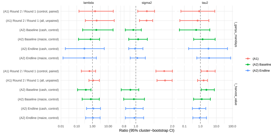
Figure 15: Variance-homogeneity tests
