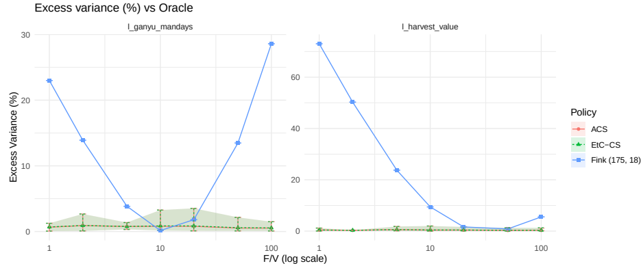
Figure 12: Excess variance across cost ratios
