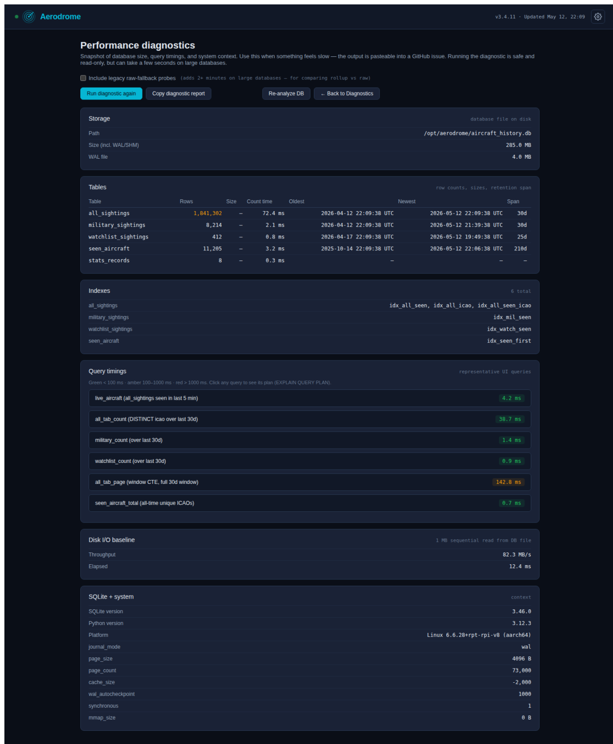
The Performance diagnostic page — storage, query plans, and auto-generated hints for constrained hardware.
