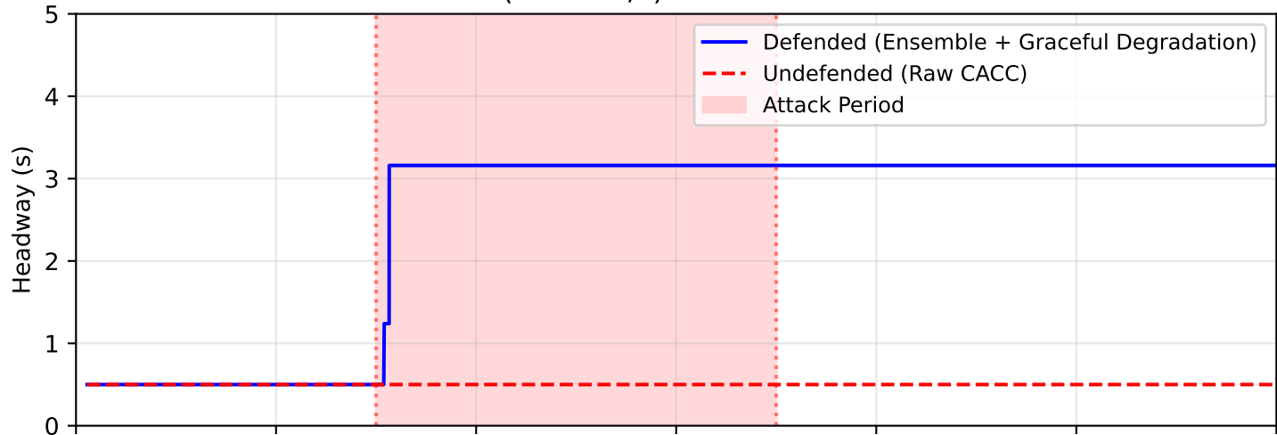
Offset Attack (+150 m/s): Defended vs Undefended
