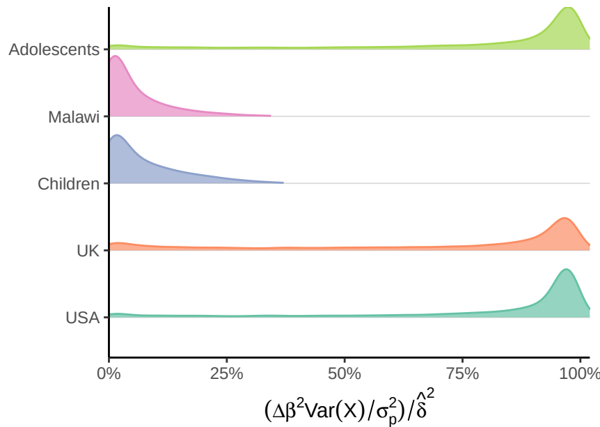
C3 Post-ComBat Effect Size
