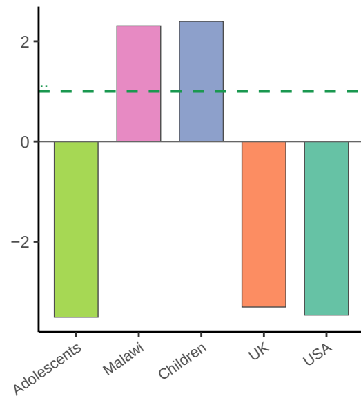
C3 Post-ComBat Effect Size
