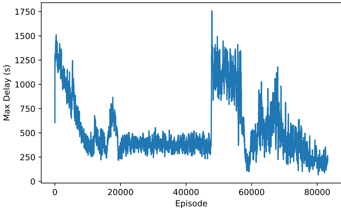
100-episode Moving Average — Max Delay
