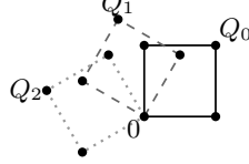
FIGURE 4. The three cross-sections Q_r of the configuration \mathcal{P} in the plane perpendicular to the common edge e . Solid, dashed, and dotted lines represent Q_0 , Q_1 , and Q_2 , respectively.
