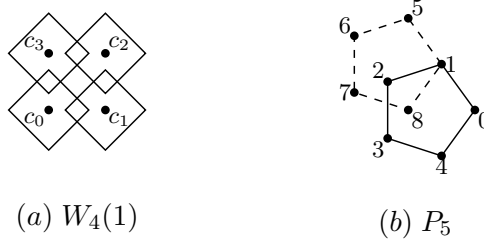
FIGURE 3. The planar configurations used for W_4(1) and P_5 .
