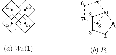
FIGURE 3. The finite planar patches used for W_4(1) and P_5 .
