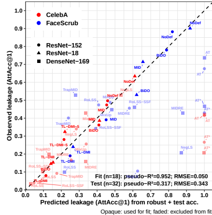
Figure 1: The privacy–robustness relationship in Torp et al. [2026] does not generalize under standard MIA evaluation. Opaque points were included in the original Torp et al. [2026] regression.
