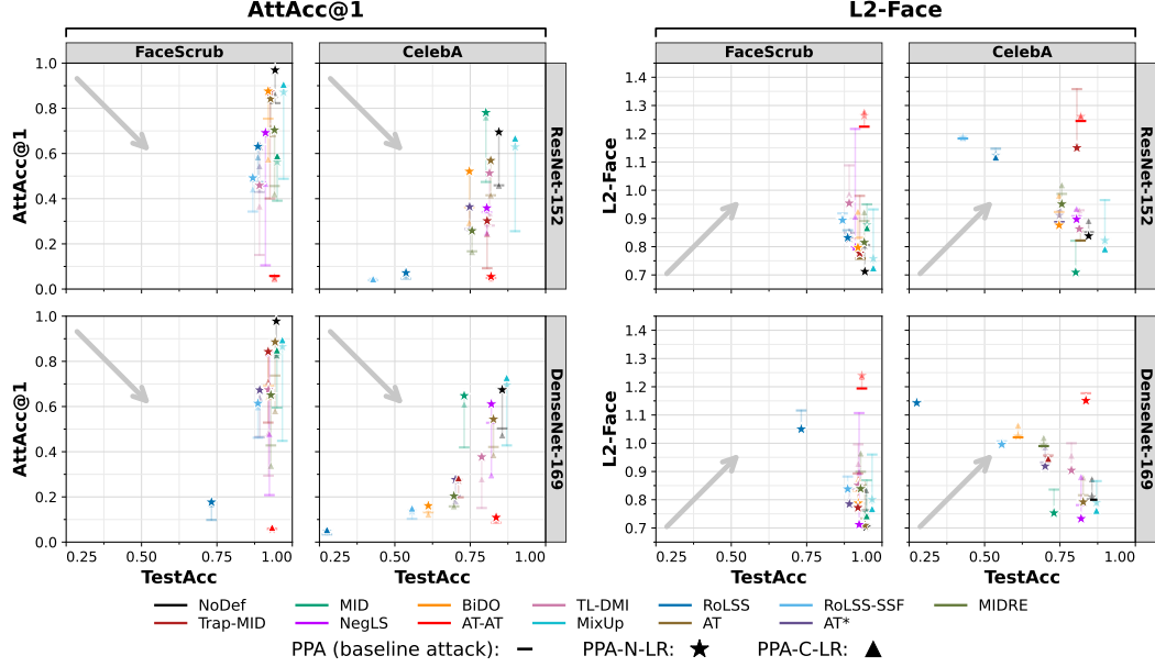
Figure 2: Leakage (AttAcc@1 & L2-Face) vs. test accuracy. Shapes denote attacks. Vertical lines measure vanilla PPA vs. the adaptive attacks, and opaque markers highlight the worst-case leakage.
