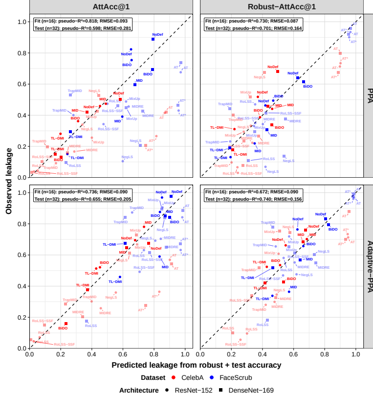
Figure 3: The privacy–robustness relationship generalizes substantially better under adaptive attacks (bottom row) and a Robust Inception-v3 evaluator (right column). Opaque points were used for fitting (the same set of defenses that were used to fit in the Torp et al. [2026] regression).
