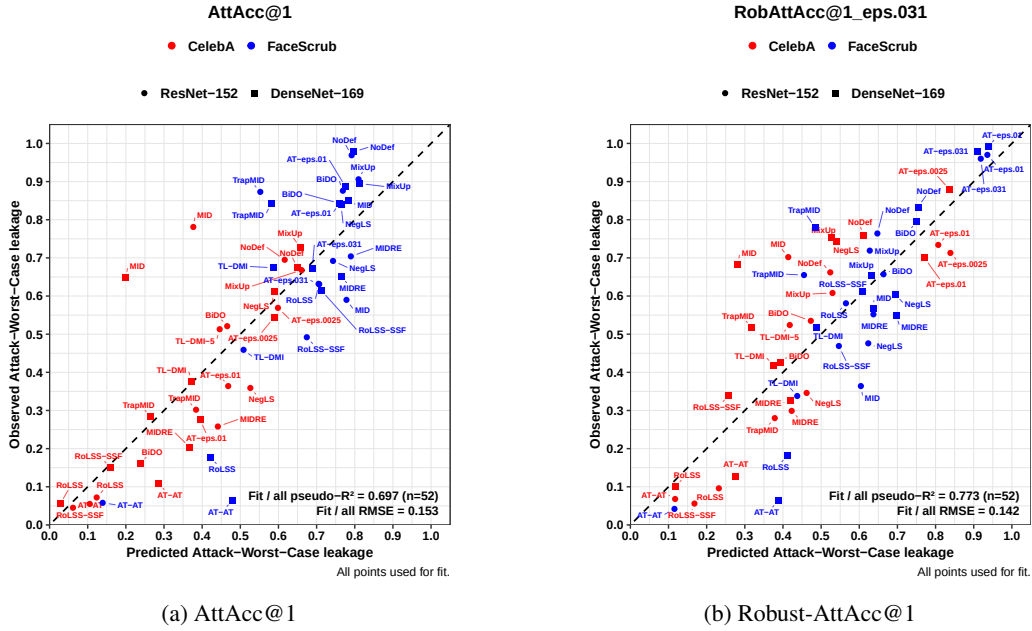
Figure 6: Regressions fit on all data points using the worst-case adaptive attack.
