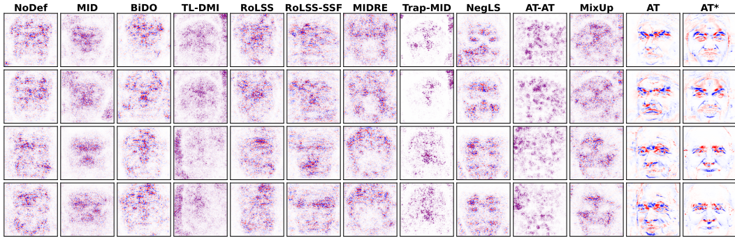
Figure 4: Heatmaps of inversion-time loss gradients \nabla_x \mathcal{L}_{\text{cls}}(x) , where x = G(z) is a GAN-generated reconstruction at various PPA iterations on ResNet-152. Gradient magnitudes are normalized , i.e., incomparable across target models. Rows 1 & 2 correspond to FaceScrub class 12 at attack iterations 9 and 49, respectively. Rows 3 & 4 correspond to the same iterations of class 16.
