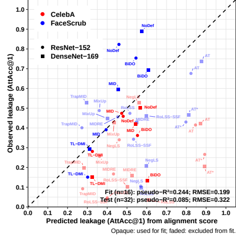
Figure 5: Regression predicting leakage from the alignment score. The fitted alignment coefficient is positive (6.16), consistent with greater alignment being associated with greater leakage, although held-out predictive fit is weak.
