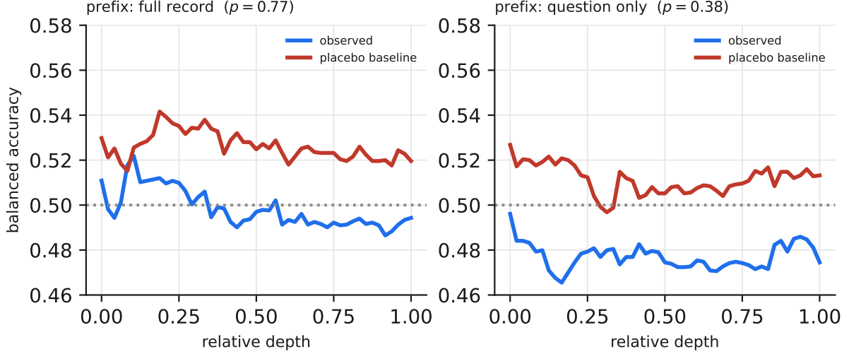
Figure 11: Phase 3, measured. Observed depth profile against the level-matched placebo baseline on Oren et al.’s contaminated 1.4B checkpoint, PIQA injected at m = 50 , under two prefix lengths. The baseline is not flat in either panel and changes shape with prefix length, which is why it has to be measured rather than assumed. Neither observed profile departs from it significantly.
