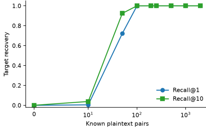
Figure 6: Known-plaintext alignment destroys the unknown-rotation assumption: with about k leaked pairs the rotation is recovered. The x axis uses a symlog scale to include m = 0 .
