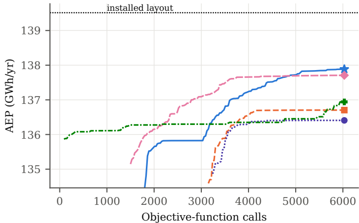
Horns Rev 1, 16 turbines: median best feasible AEP
