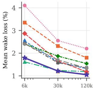
Data Set II, r = 1000 m, N = 15
