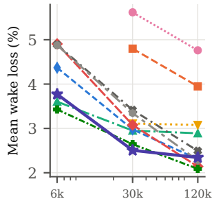
Data Set II, r = 750 m, N = 12
