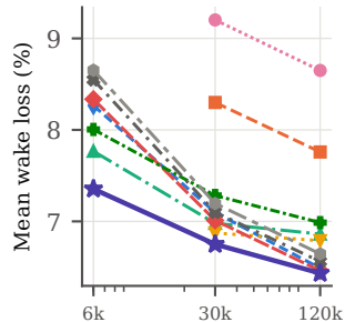
Data Set II, r = 500 m, N = 10
