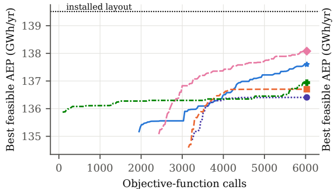
Horns Rev 1, 16 turbines
