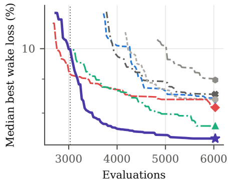
Data Set II, r = 500 m, N = 10
