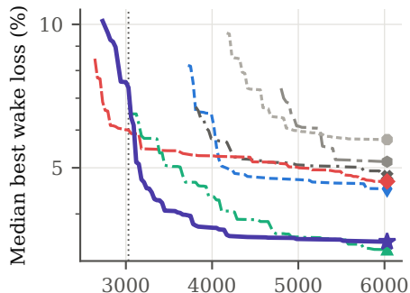
Data Set II, r = 500 m, N = 10
