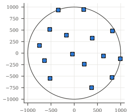
Data Set II, r = 1000 m, N = 15 best of all methods: MS-SLSQP (0.289 pp)
