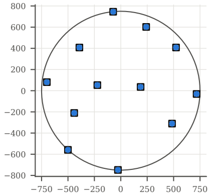
Data Set II, r = 750 m, N = 12 best of all methods: SSA-VNS
