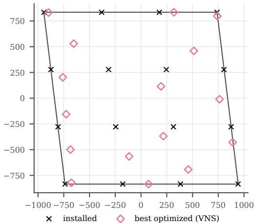
Horns Rev 1, 16 turbines (m)
