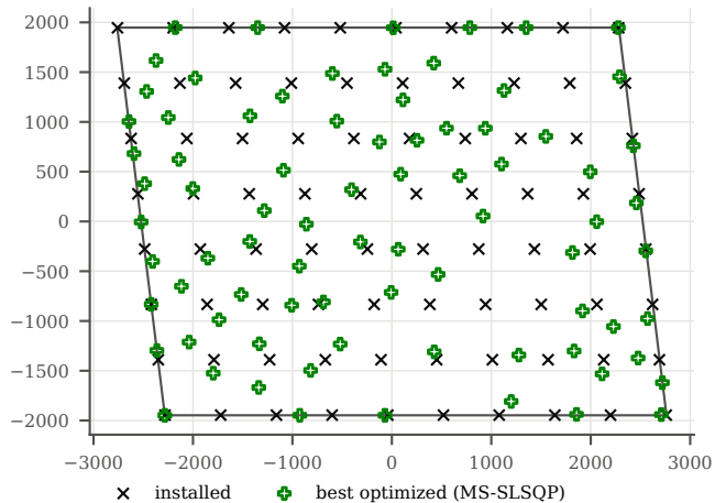
Horns Rev 1, 80 turbines (m)
