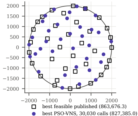
IEA37 CS1, 36 turbines (AEP in MWh)
