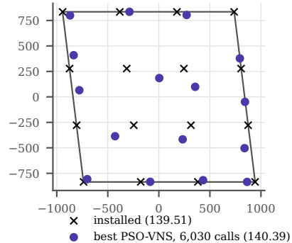
Horns Rev 1, 16 turbines (AEP in GWh/yr)
