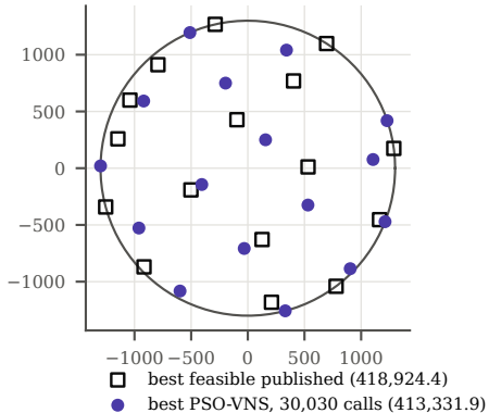
IEA37 CS1, 16 turbines (AEP in MWh)
