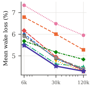
DS II, r = 750 m, N = 12
