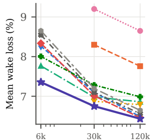
DS II, r = 500 m, N = 10
