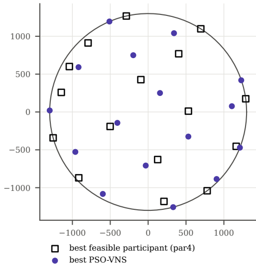
IEA37 CS1, 16 turbines (m)
